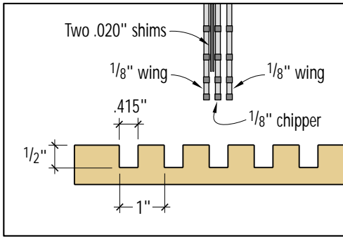
Dado stack setup detail
